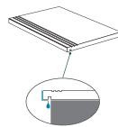
USTEPD 12x24 (2cm) Step Tread w/ Grooves & Drip Flap
